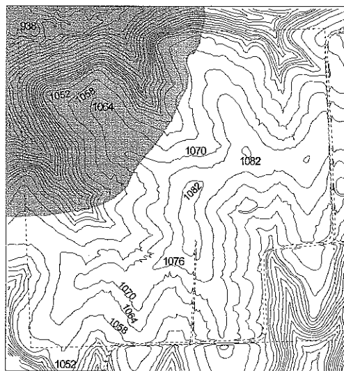
Figure 3. Topographic map of Rockefeller Experimental Tract showing elevations (6-foot contour intervals) and distribution of presettlement forest (shaded area, as determined from General Land Office plat map of 1860). Refer to Fig. 1 for orientation, scale, and cultural features.
