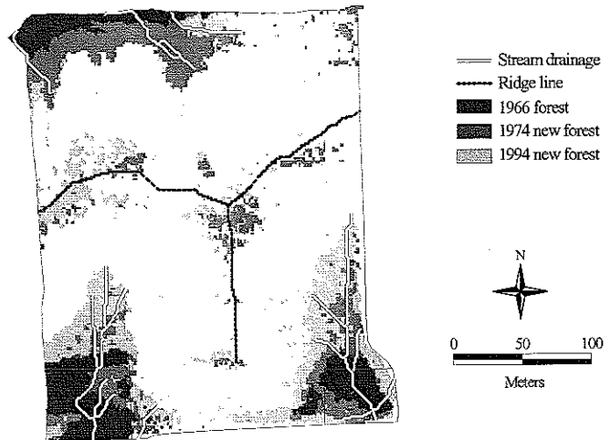
Figure 6. Forest cover changes in an untreated area (units E, F, and K, Fig. 2) of the Rockefeller Experimental Tract. Change in forest cover (1966 baseline) shown as new forest in 1974 and 1994.
